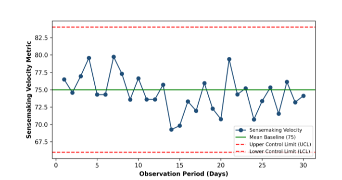
Figure 30 Description & Analytical Context: Statistical Process Control (SPC) chart proving organizational sensemaking velocity remains stable within control limits.
