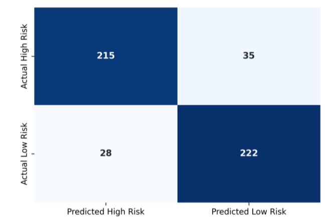
Figure 25 Description & Analytical Context: Confusion matrix indicating 87.4% overall classification accuracy for strategic risks.
