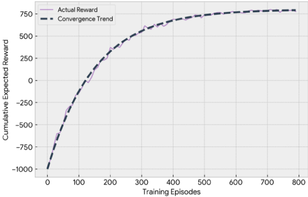
Figure 17: Deep Reinforcement Learning (DRL) convergence reward curve over training episodes. Visualization Explanation 7: The Multi-Objective DRL agent achieves policy stability by Episode 600, balancing capital expenditures against operational disruption mitigation. The convergence trend demonstrates robust learning in the simulated environment.
