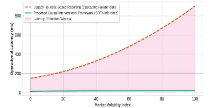
Figure 8: Operational inference latency and cascade prevention performance across market volatility index levels.
