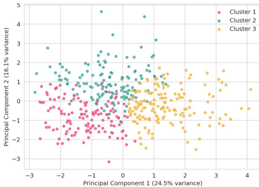
Figure 6. K-means cluster solution of teacher AI-readiness profiles in principal-component space.
