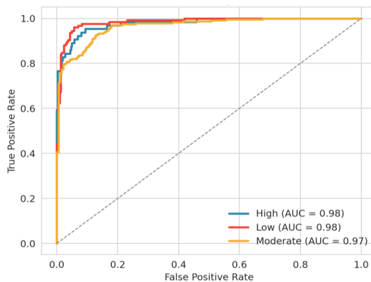
Figure 4. One-vs-rest ROC curves for the random forest classifier across readiness levels.
